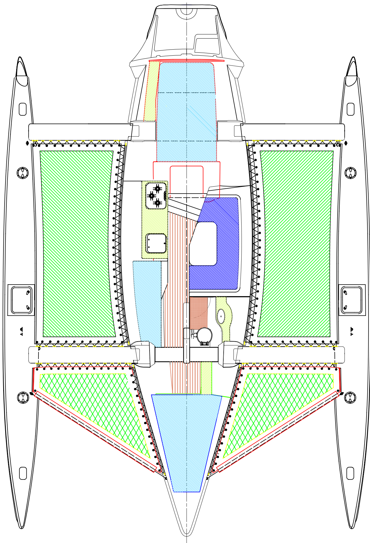
- ACCOMMODATION PLAN - CORSAIR 37CR/37RS
