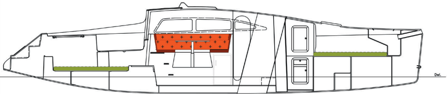
Corsair 36 Inboard Profile and Accommodation Plan
